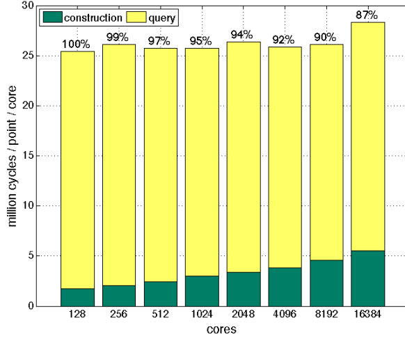
FIG. 3.2. Weak scaling of RKDT on Stampede: Weak scaling of all nearest neighbors in 10 iterations of RKDT on Stampede. We use 1024 dimensional normal distribution data with k = 2048 . 50,000 points per process are used; one process per socket with 8 threads. The percentages represent the relative efficiency of each run normalized to the 128-core run.
