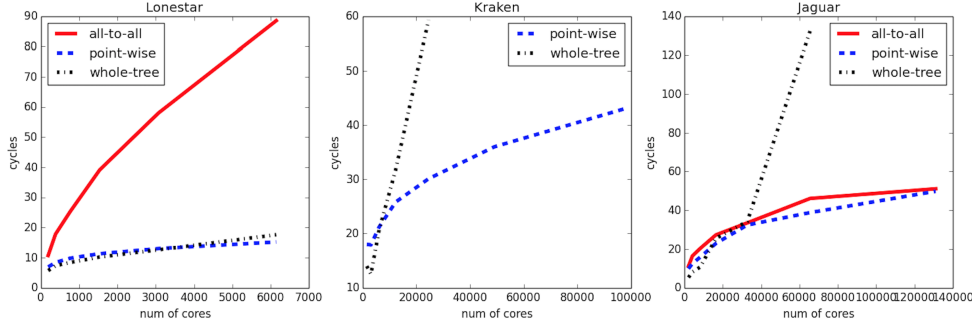
FIG. 3.1. Weak scaling of construction only for RKDT on Lonestar, Kraken, and Jaguar respectively: The metric used to compare across platforms is millions of cycles / point / core, i.e., the number of clock cycles that would be needed to perform the query for each point using only a single core.
