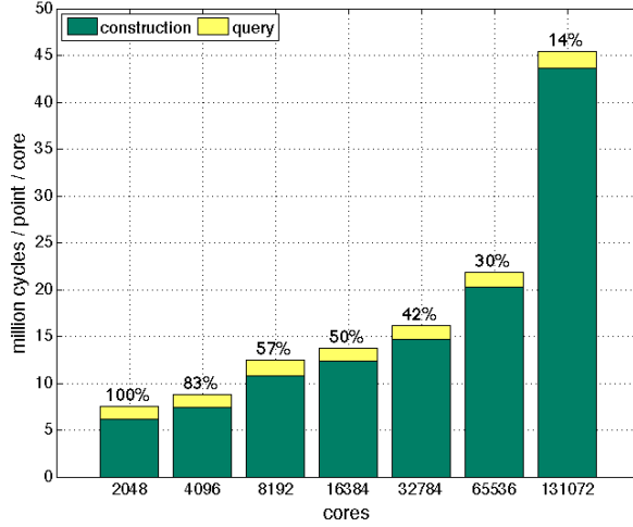
FIG. 3.3. Weak scaling of RKDT on Jaguar: Weak scaling of all nearest neighbors in 8 iterations of RKDT on Jaguar. We use 2048 dimensional normal distribution data with k = 2048 . 50,000 points per process are used; one process per socket with 8 threads. The percentages represent the relative efficiency of each run normalized to the 2,048-core run.
