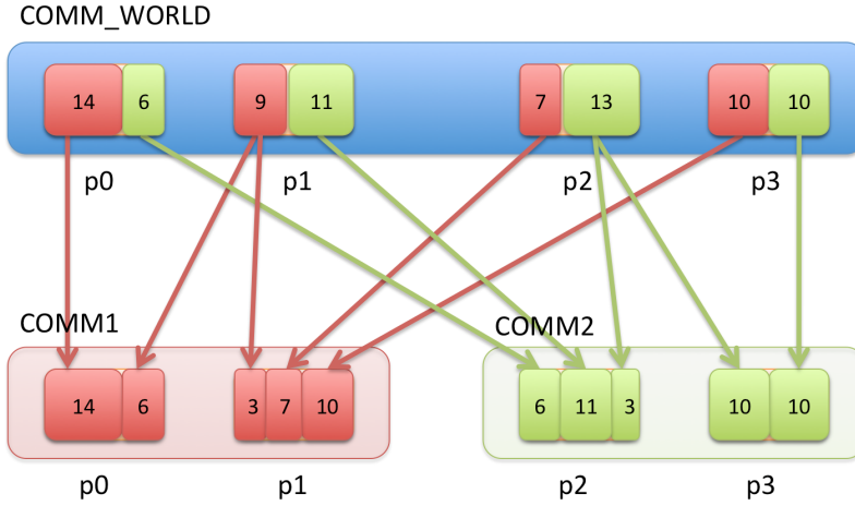
FIG. 2.4. Here we illustrate the problem of load balancing when we split a node and its communicator. The blue region (with communicator COMM_WORLD ) denotes the parent. Notice that every process in COMM_WORLD has an equal number of points. After the hyperplane split, some points go to the left child (red) and some to the left child (green). Also, we need to split COMM_WORLD to COMM1 and COMM2 , assign processes to each communicator, and redistribute the points from the parent to the children. There is no unique way to do this, but the goal is that upon completion each process in COMM1 and COMM2 has again the same number of points with as little communication as possible. Using an MPI_Alltoallv() is one possible way to do it.
